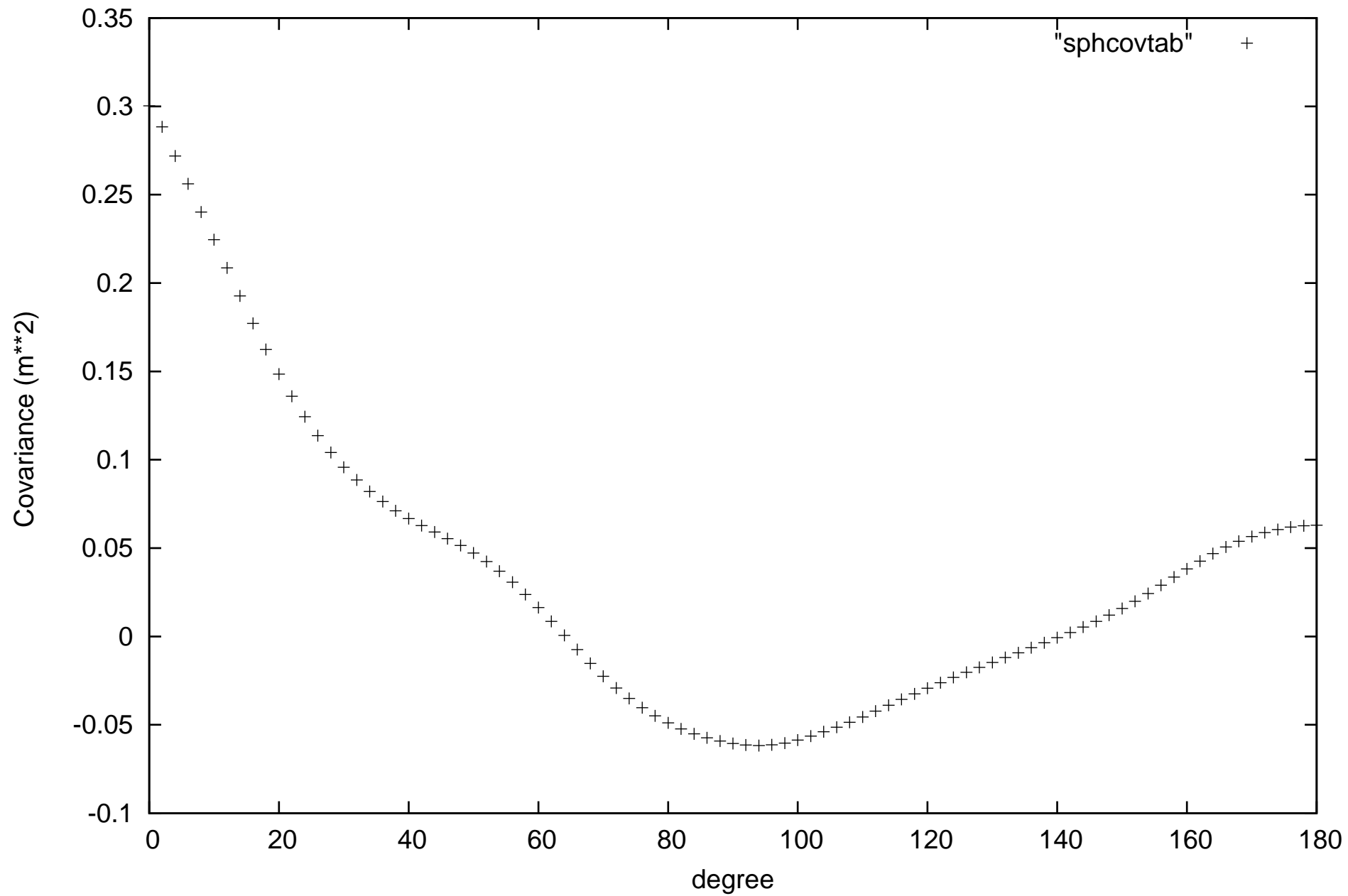
Covariance function
