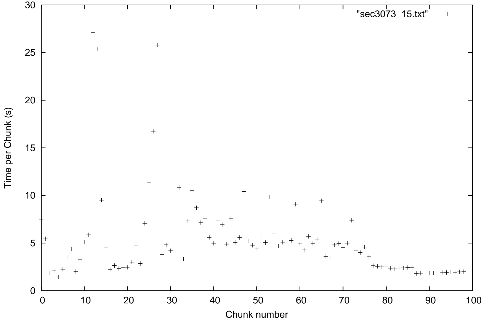
time for 15 block-size
