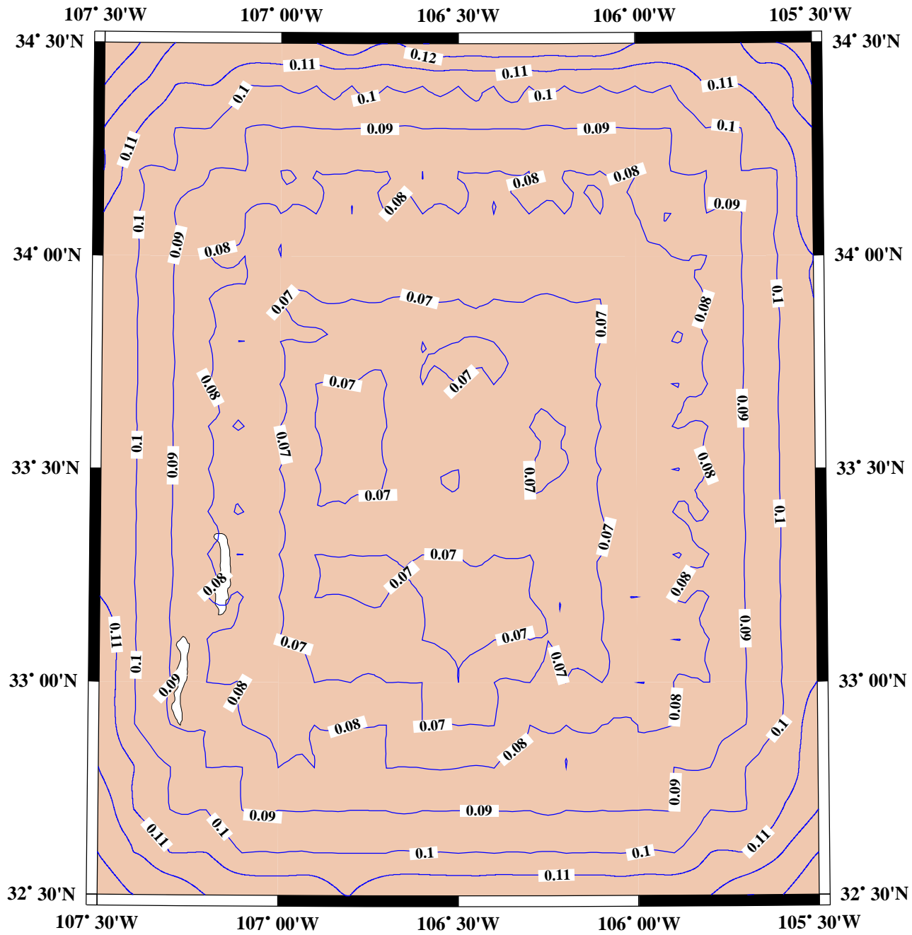
Figure 7. Errors of reduced height anomalies / m
