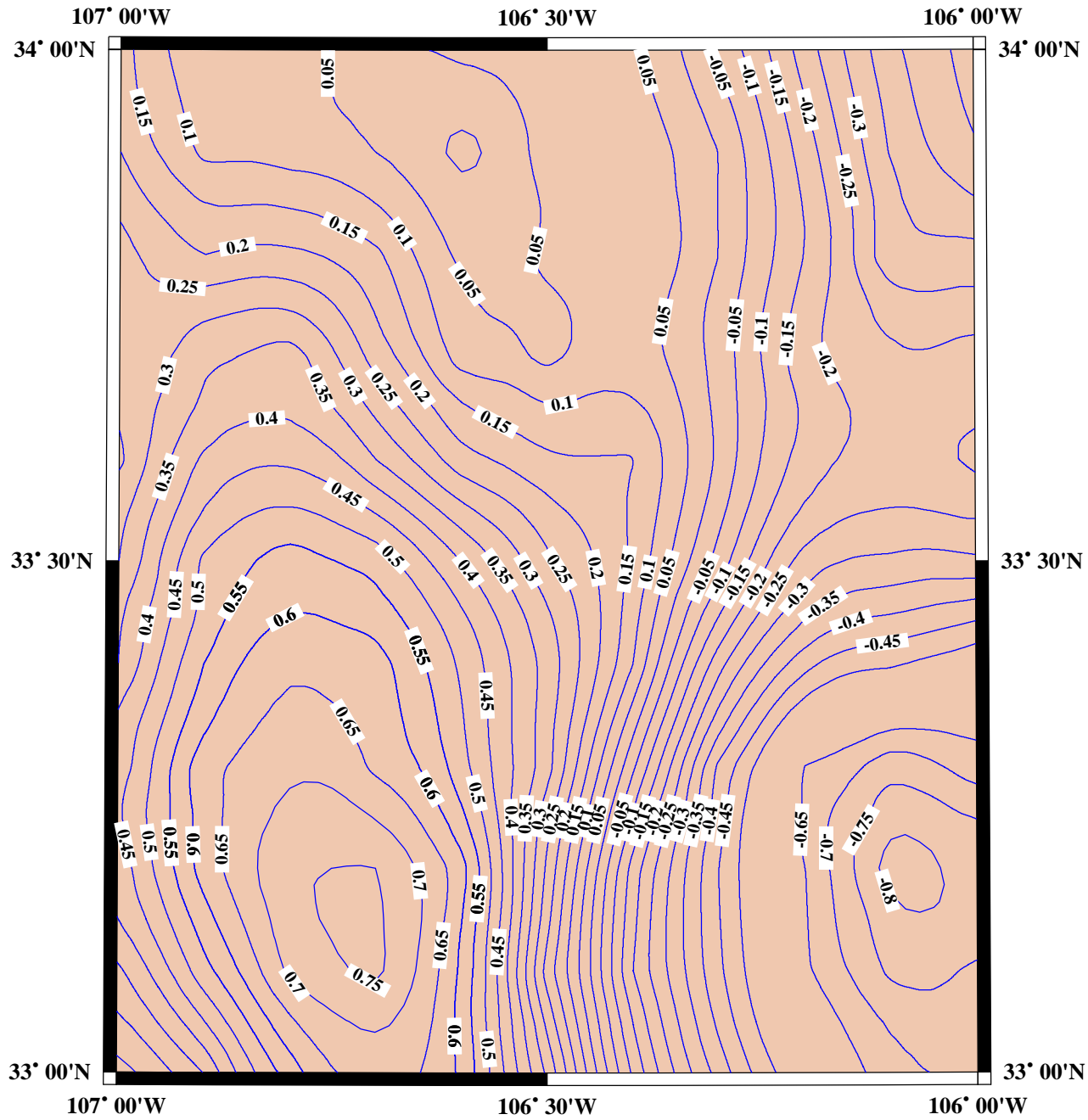
Figure 6. Reduced height anomalies / m
