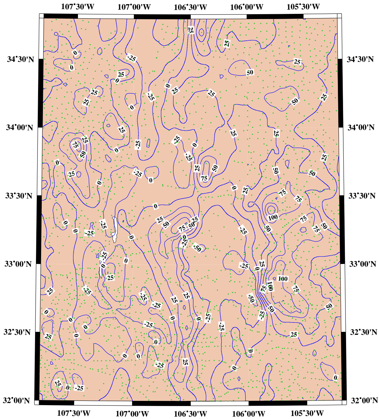
Figure 2. Free-air gravity anomalies / mGal
