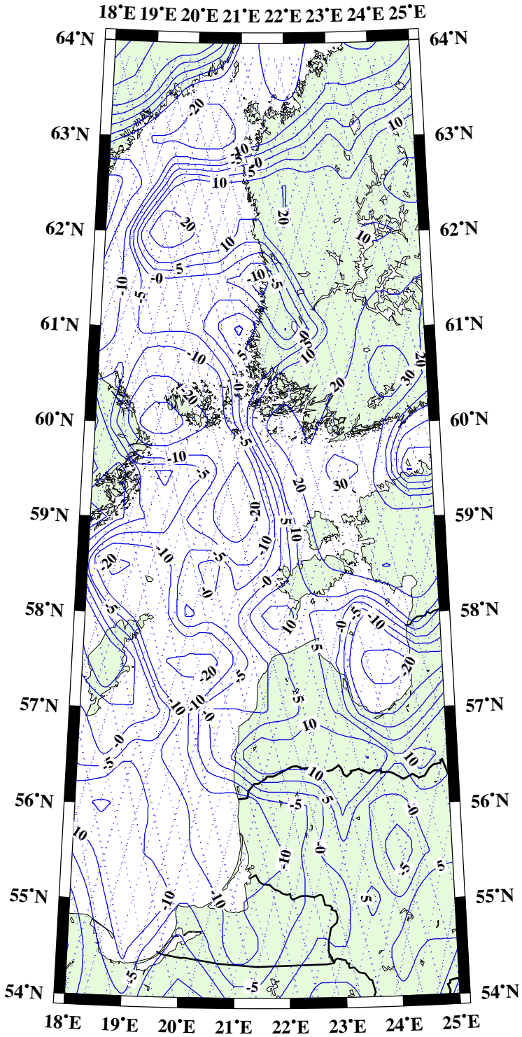
GOCE dgs diff. (mgal) from Tyy in central Fenno-Scandia.
