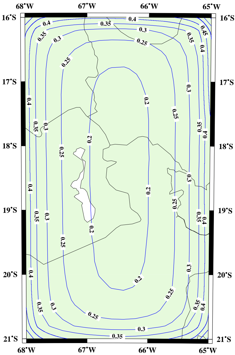
Height anomaly error estimates from CHAMP and gravity data / m
